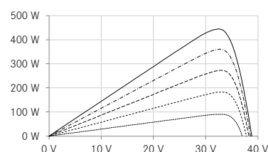
UP-Kennlinie Bsp. 445 Wp
