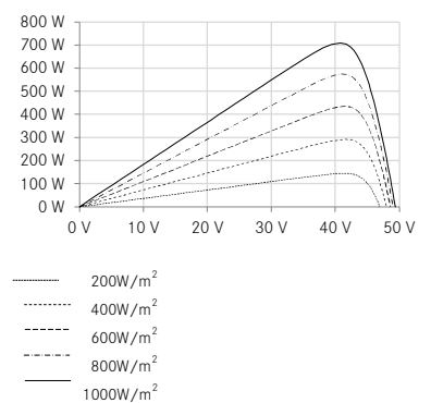
UP-diagram e.g. 710 Wp
