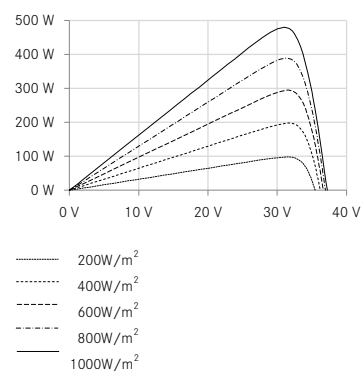
UP-diagram e.g. 480 Wp
