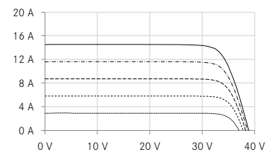
UP-Kennlinie Bsp. 445 Wp
