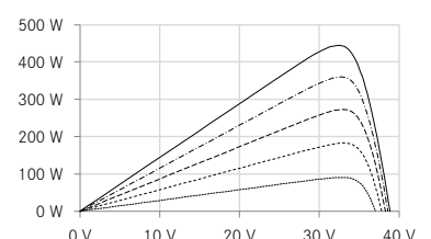
UP-Kennlinie Bsp. 445 Wp
