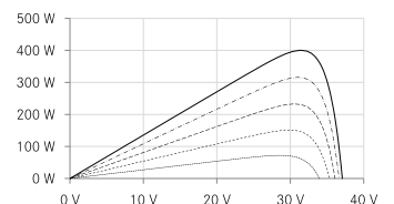
UP-Kennlinie Bsp. LX-400M / 182-108+
