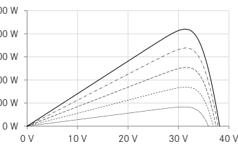
UP-Kennlinie Bsp. 420 Wp
