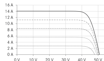
UP - diagram e.g. 560 Wp
