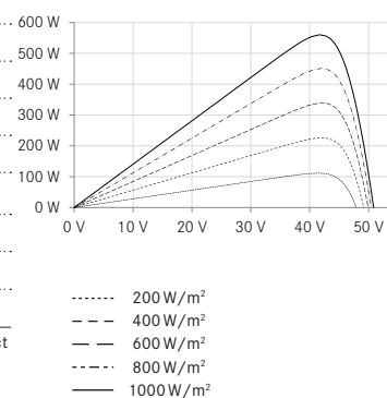
UP - diagram e.g. 560 Wp
